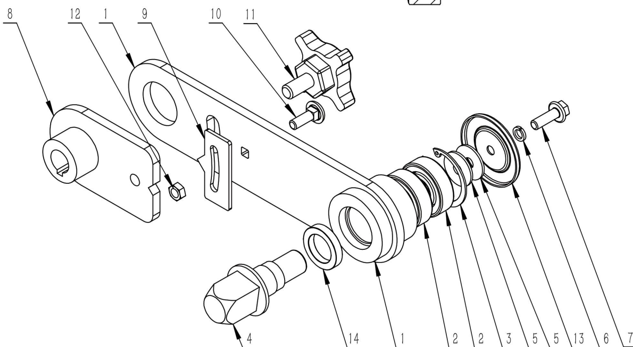
Left sync plate assembly
