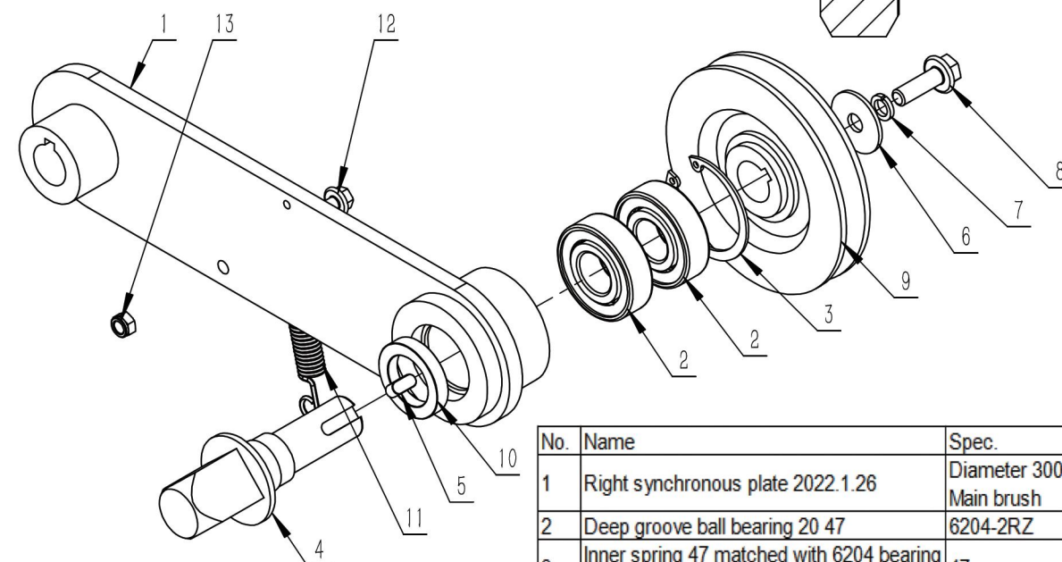
Right sync plate assembly
