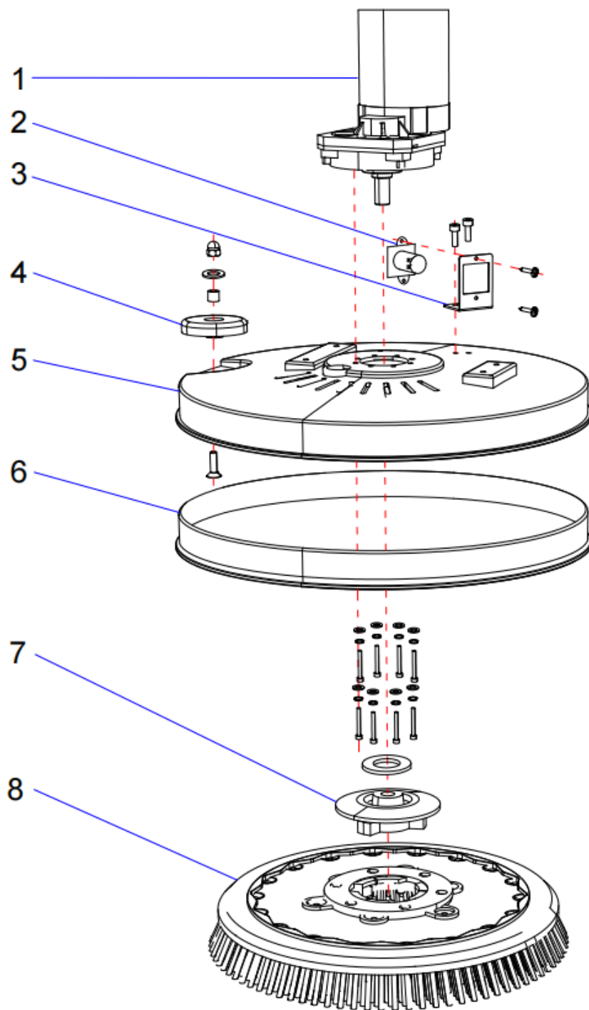
Brush plate parts
